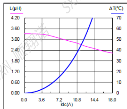
SMMS1040-3R3M
