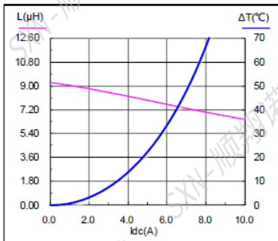
SMMS1040-330M
