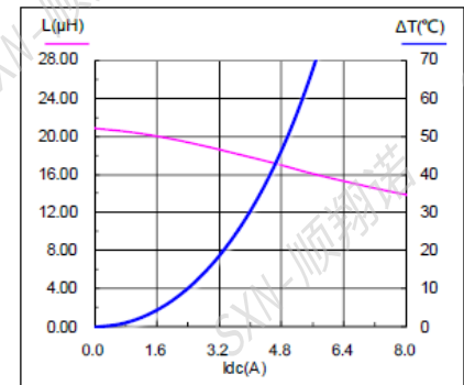
SMMS1040-680M
