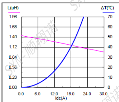
SMMS1040-1R5M
