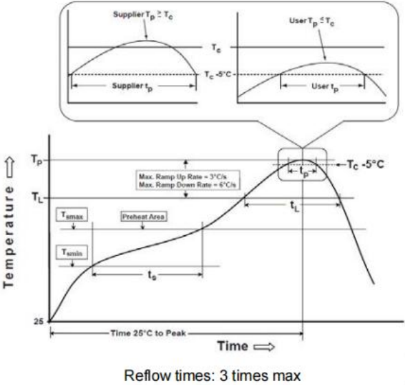
Fig.1 Soldering Reflow
