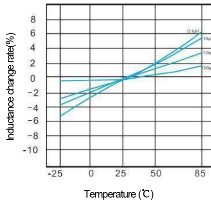
Inductance change rate vs. Temperature Characteristics
