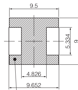
Series PCC-M0840M-LP (ETQP4M□□□KVK)
