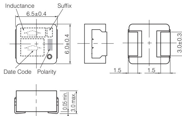
Series PCC-M0630M-H (ETQP3M□□□HFN)
