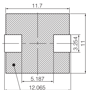
Series PCC-M1040M-LP (ETQP4M□□□*KVC) * Exemption "1R0"
