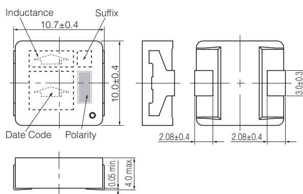
Series PCC-M1040M-LP (ETQP4M□□□*KVC) * Exemption "1R0"
