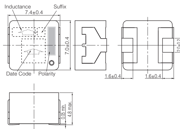
Series PCC-M0748M-LE (ETQP4M□□□KFM)
