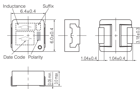
Series PCC-M0630M-LP (ETQP3M□□□KVN)
