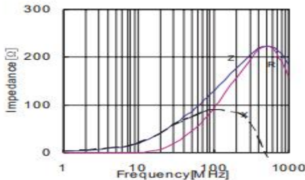
产品特性曲线图：Product Characteristic Curve
